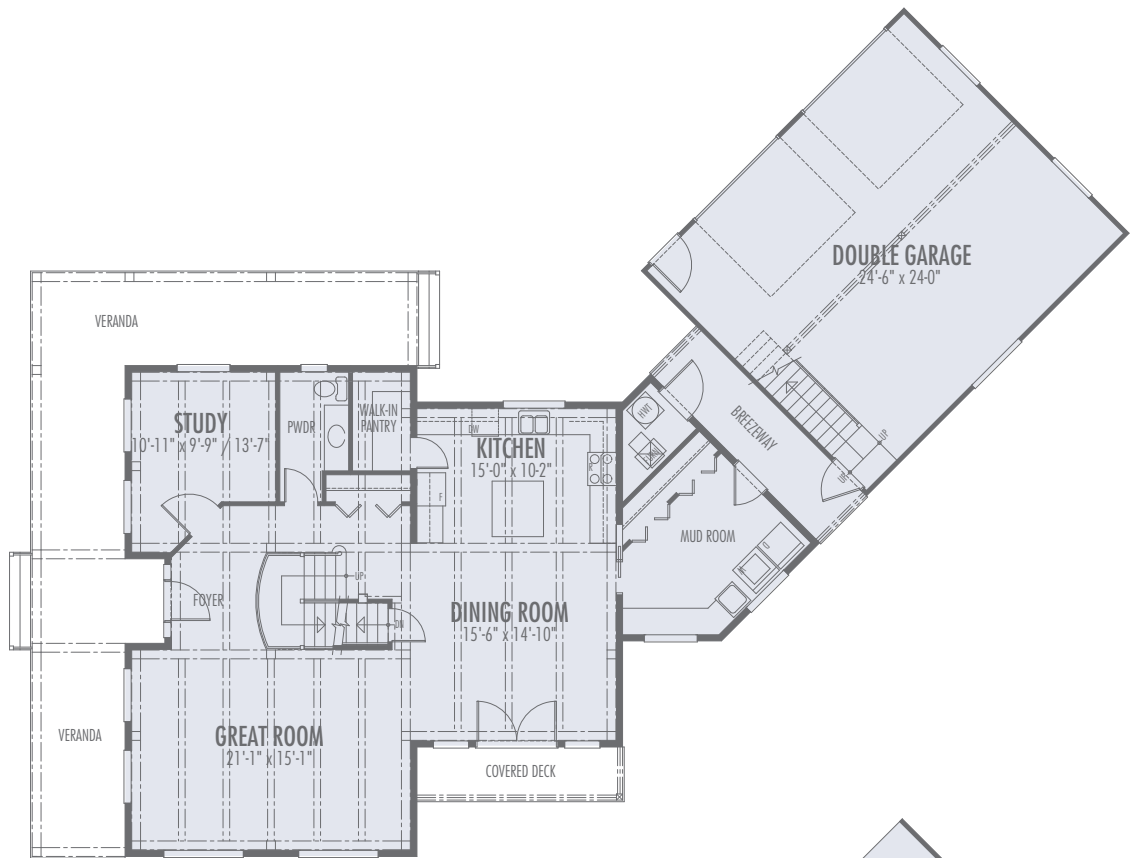
Main Floor
