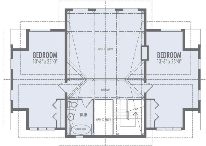
Upper Floor
