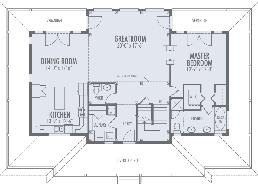
Main Floor
